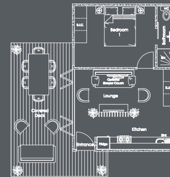
X-30 PLAN OPTION 1
