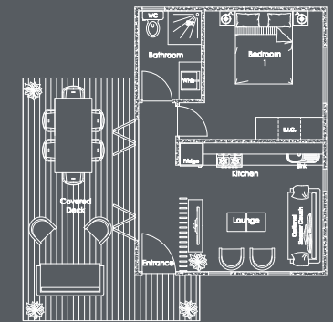
X-30 PLAN OPTION 2
